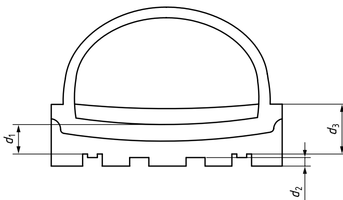
Figure 39 — All-rubber and all-polymeric footwear (cleated)
