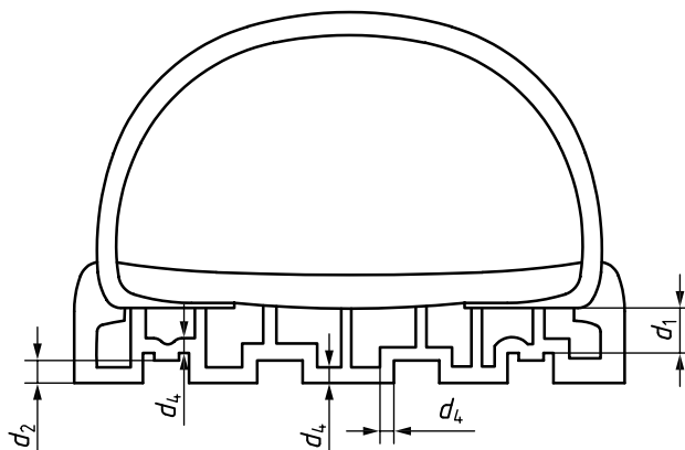
Figure 40 — Cemented footwear (minimum thickness)
