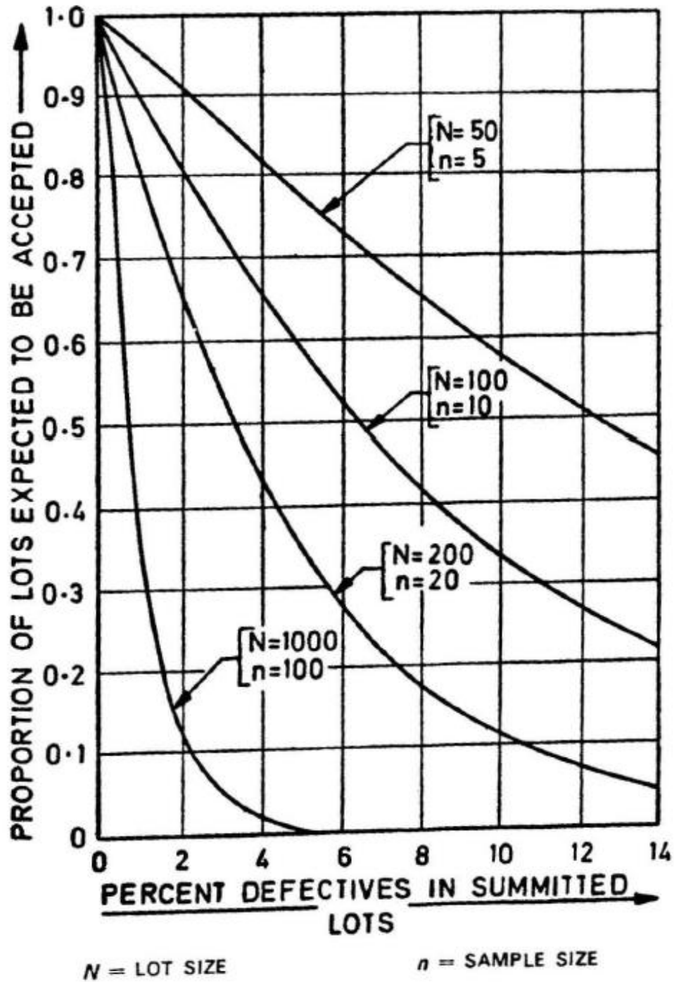
FIG. 5 SOME OC-CURVES FOR PERCENTAGE SAMPLING
