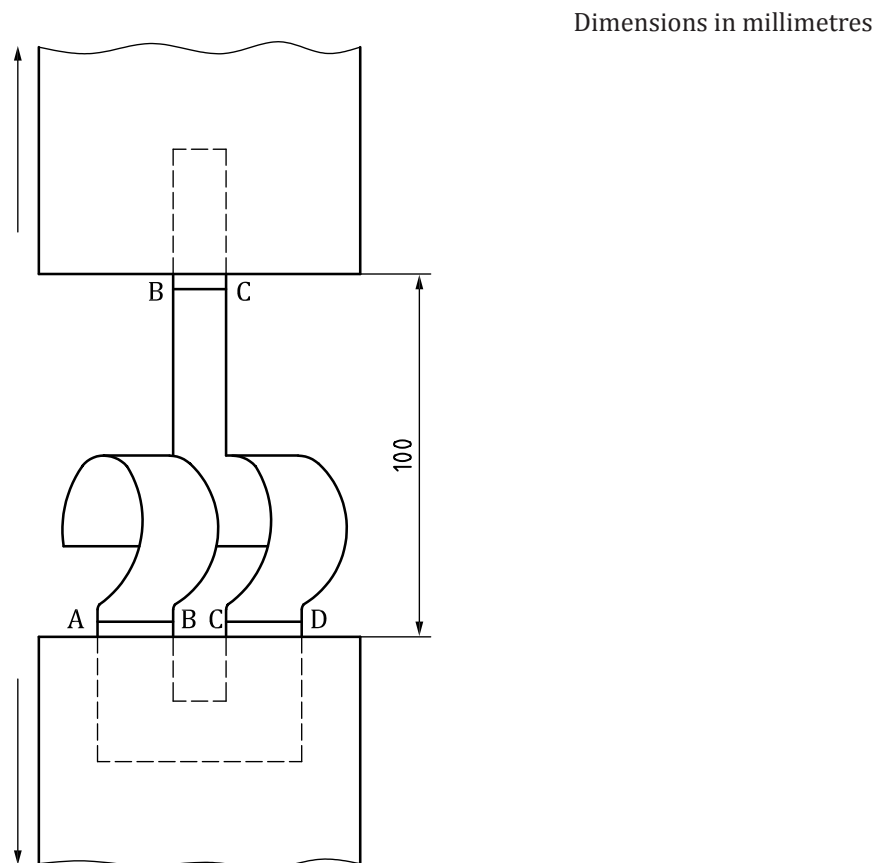
Figure 3 — Method of clamping tongued test piece
