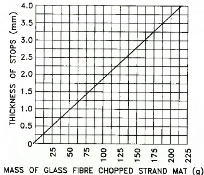
FIG. 2 MASS OF GLASS FIBRE CHOPPED STRAND TO PRODUCE 300 mm \times 275 mm LAMINATE WITH A GLASS CONTENT OF 42.5 PERCENT BY MASS
