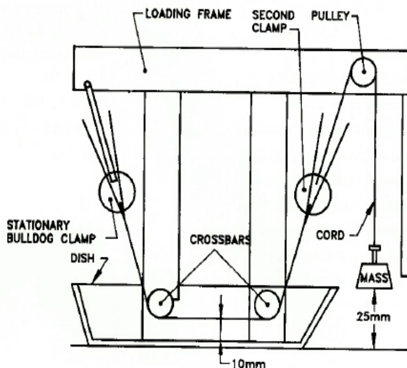
FIG. 4 APPARATUS FOR THE DETERMINATION OF MAT BINDER SOLUBILITY
