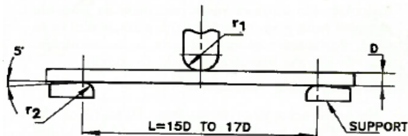
FIG. 1 ARRANGEMENT OF TEST SPECIMENS
