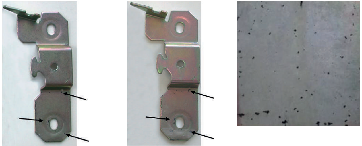
a) Part after 168 hrs NSS testing
