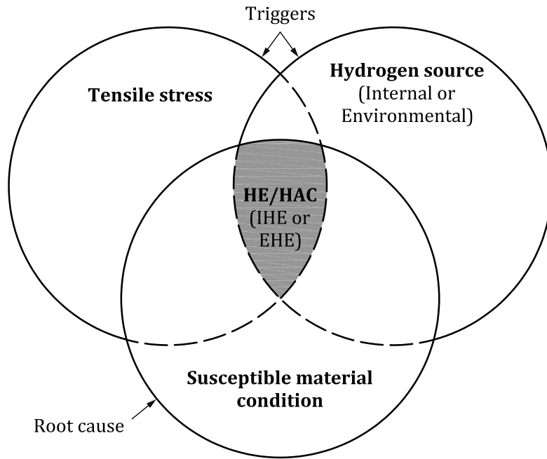
Figure B.1 — Conditions for Hydrogen Embrittlement (HE/HAC) failure
