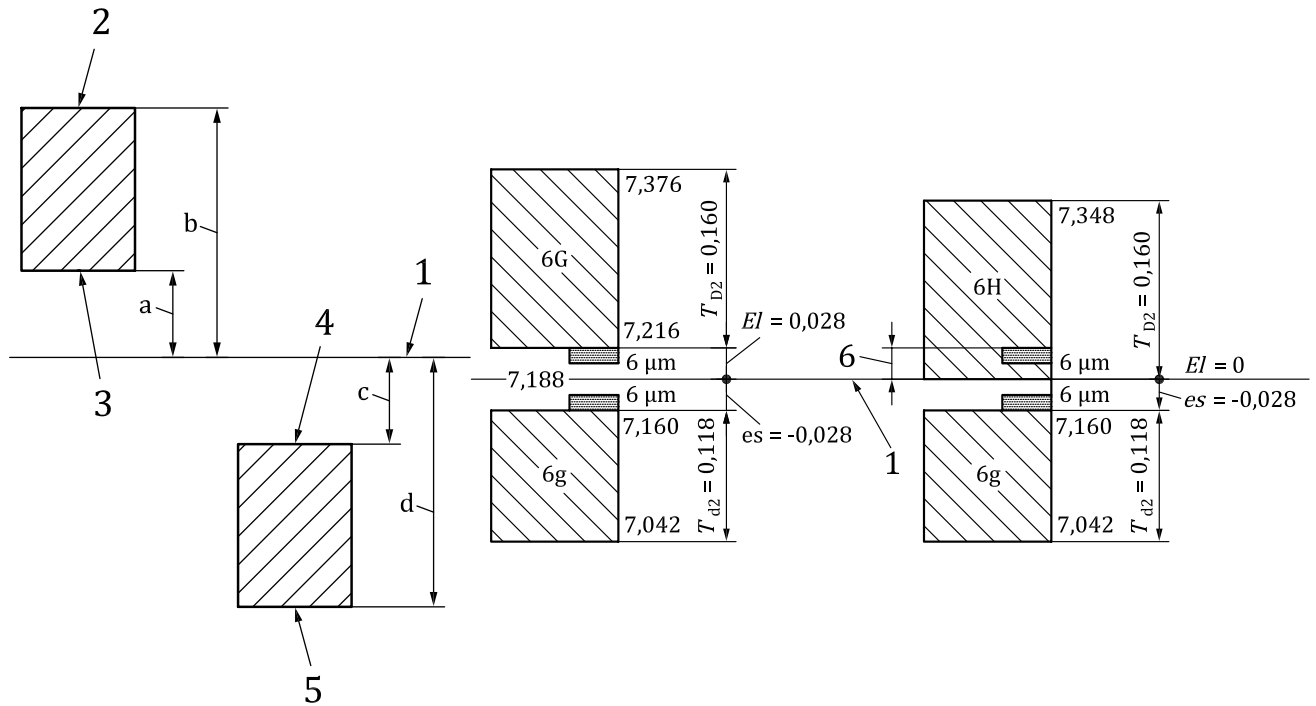
a) Internal/external thread
