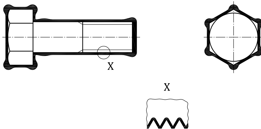
Figure D.3 — Typical distribution of coating thickness on a bolt resulting from electroplating process (exaggerated for illustrative purposes)
