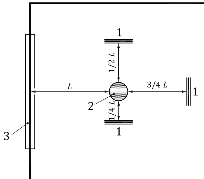
Figure E.2 — Centred spray cabinet
