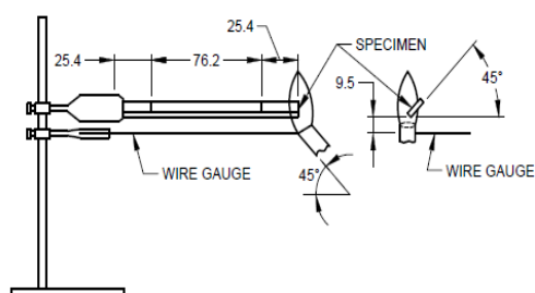
All dimensions in millimetres.
