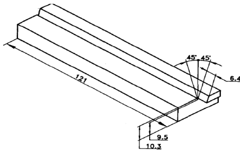
All dimensions in millimetres. FIG. 4 FLEXIBLE SPECIMEN SUPPORT FIXTURE
