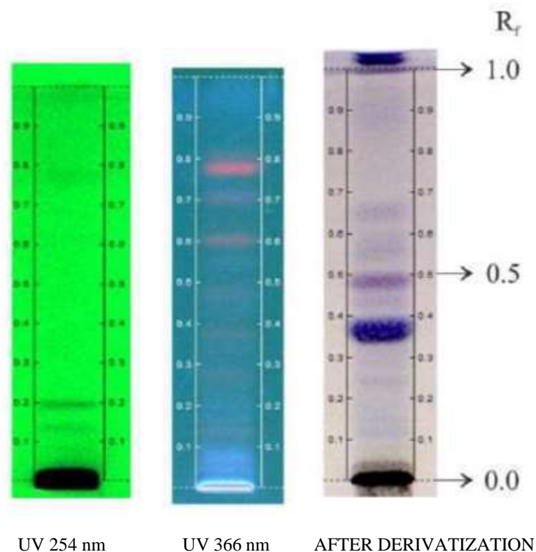
FIG. 2 TLC FINGERPRINTS OF GULNĀR FĀRSĪ ( Punica granatum L.) FLOWER
