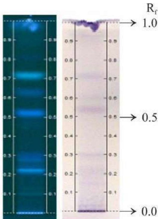
UV-366nm After derivatization
