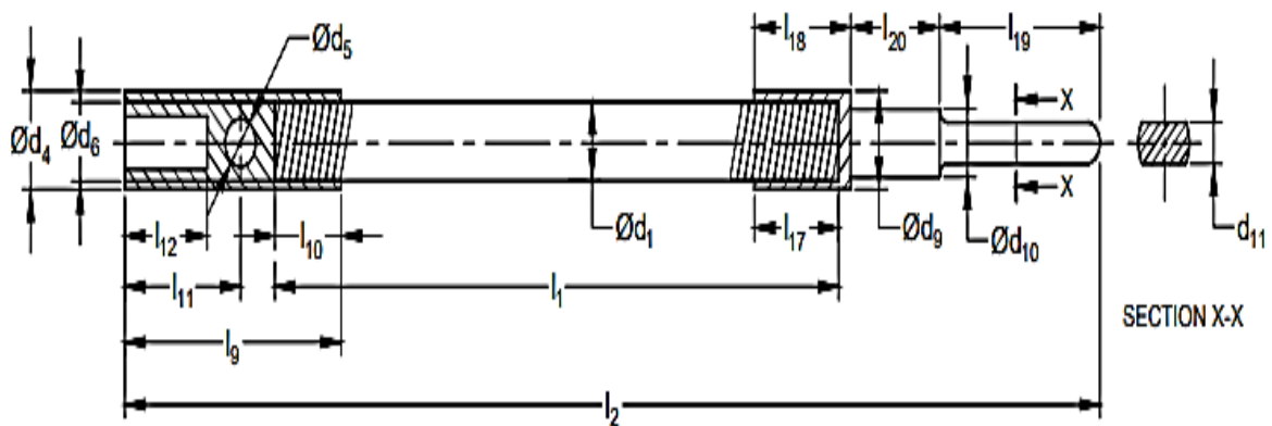
INNER SHAFT ASSEMBLY
