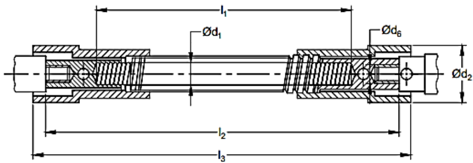
FLEXIBLE SHAFT ASSEMBLY
