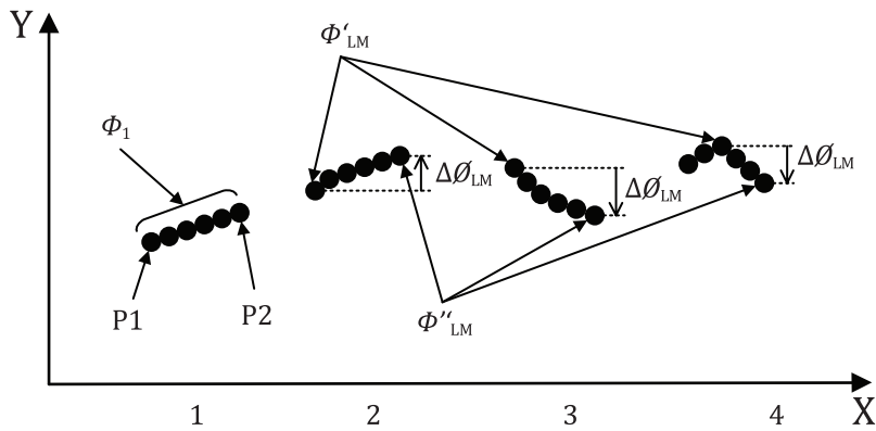
Figure 13 — Constellation plot during part of the PICC response, depicting \phi_{LM}
