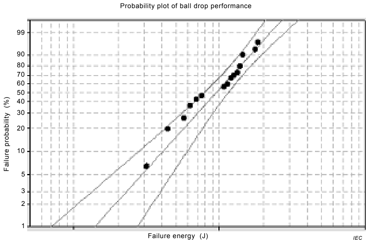
Figure 4 – Example Weibull plot
