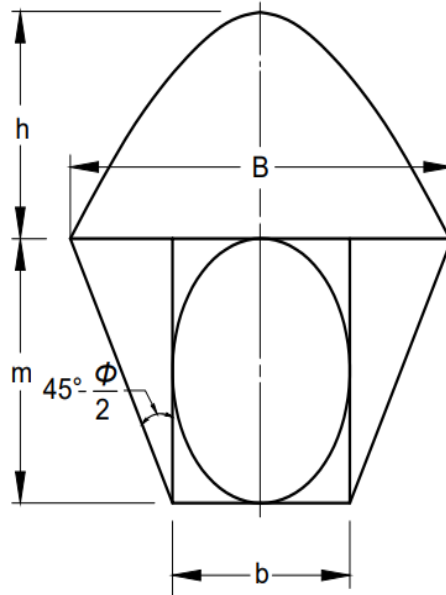
FIG. 5 ASSUMED ROCK LOAD ON A CIRCULAR CAVITY
