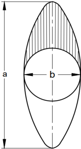
FIG. 4 FENNER'S ELLIPSE
