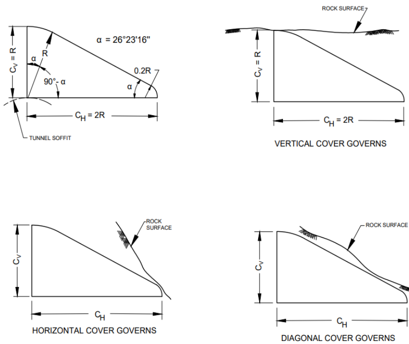
FIG. 2 ESTIMATION OF EFFECTIVE COVER
