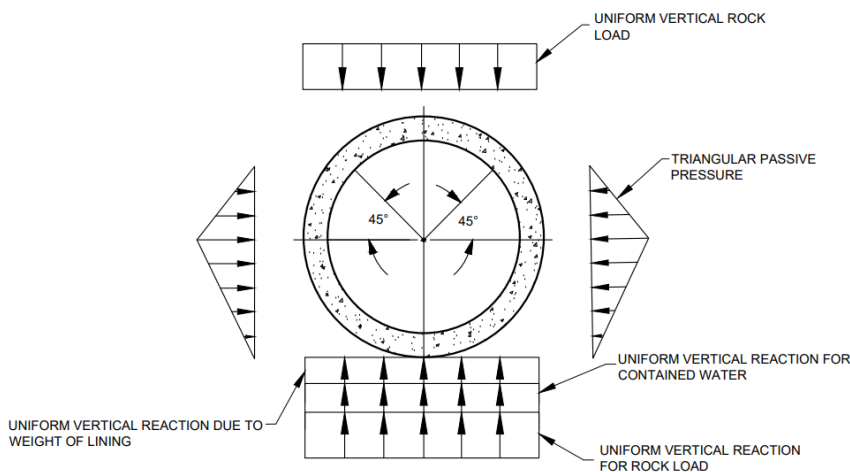
FIG. 3 EXTERNAL LOADS ON LINING
