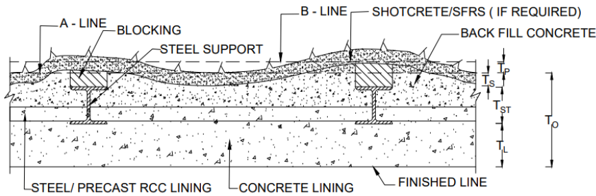
TYPICAL X-SECTION (WITH STEEL SUPPORT)
