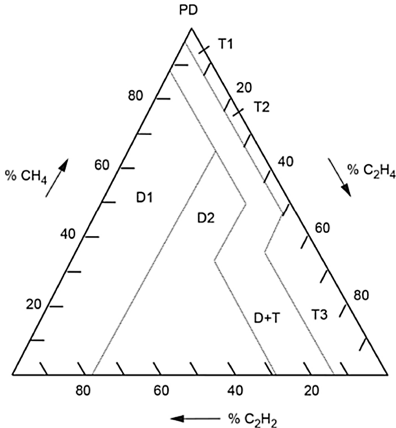
Fig. 1. Duval's Triangle 9
