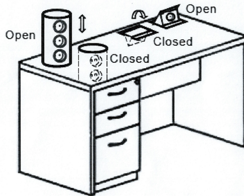
Figure 101 – Examples of socket-outlets for furniture classified according to 7.2.3.4 in open and closed positions.
